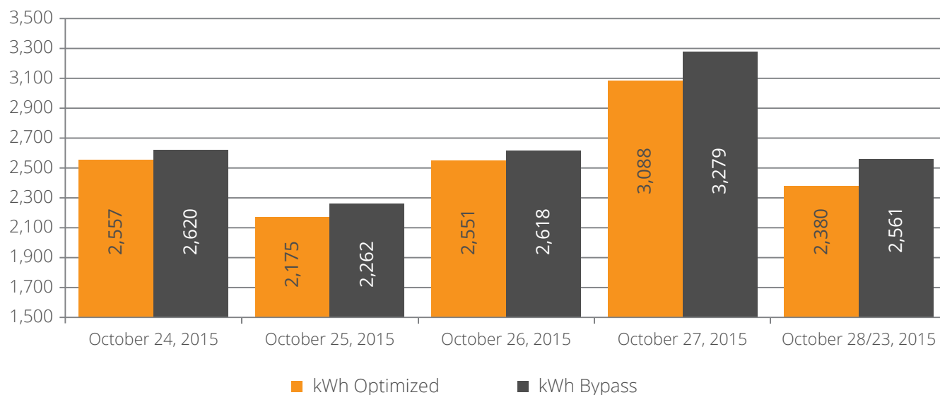
Measured Energy Usage – Before and After: (Optimized vs. Bypass)
