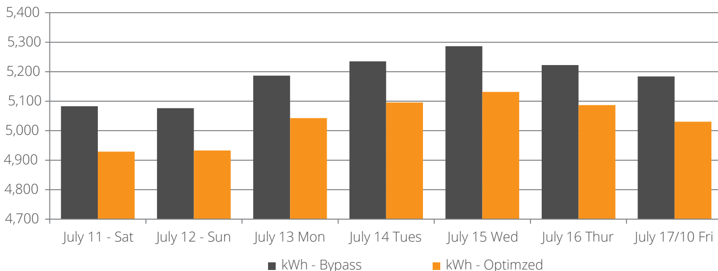
Measured Energy Usage by Day - July 2015: Bypass Voltage vs. Optimized Voltage
