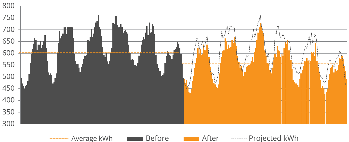
Measured Energy Usage - One Week: Voltage Before and After
