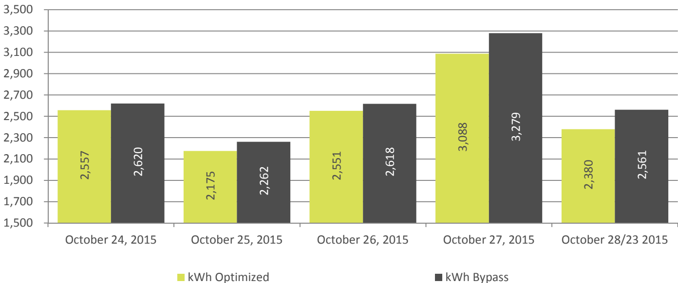
Measured Energy Consumption, Before and After: (Optimized vs. Bypass)
